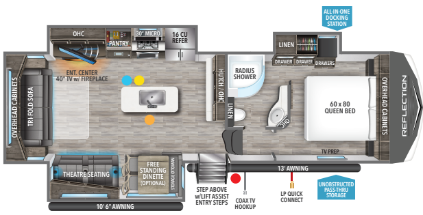
303RLS UVV 1 9,854 HITCH 1 1,865 LENGTH 2 32' 10" HEIGHT 3 12' 3" CAPACITY 74 87 47
