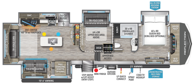
367BHS UVV 1 12,552 HITCH 1 2,461 LENGTH 2 41' 0" HEIGHT 3 12' 8" CAPACITY 74 94 47
