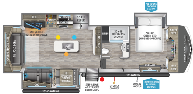
337RLS UVV 1 10,838 HITCH 1 2,185 LENGTH 2 35' 7" HEIGHT 3 12' 6" CAPACITY 74 87 47
